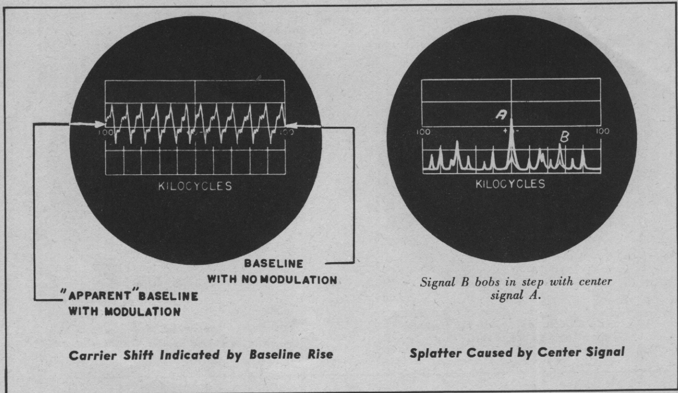
Figure 22. Carrier Shift and Splatter.
