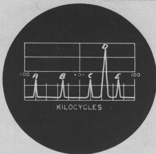
Figure 29. Frequency Setting with a Crystal Standard
