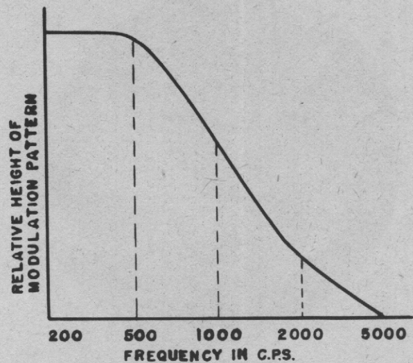
Figure 18. Variation of Height of Modulation Pattern Against Modulating Frequency
