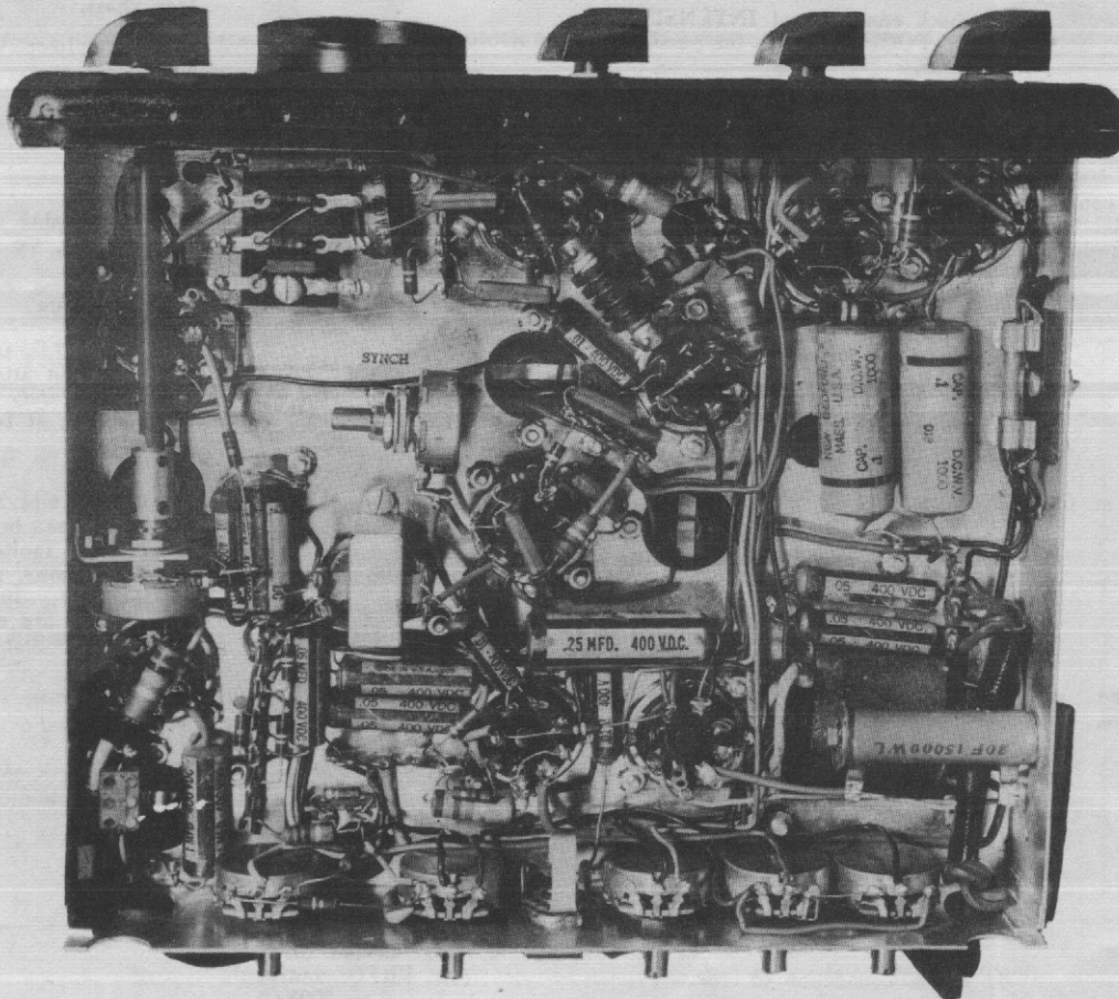
Figure 35. Bottom View of Chassis
