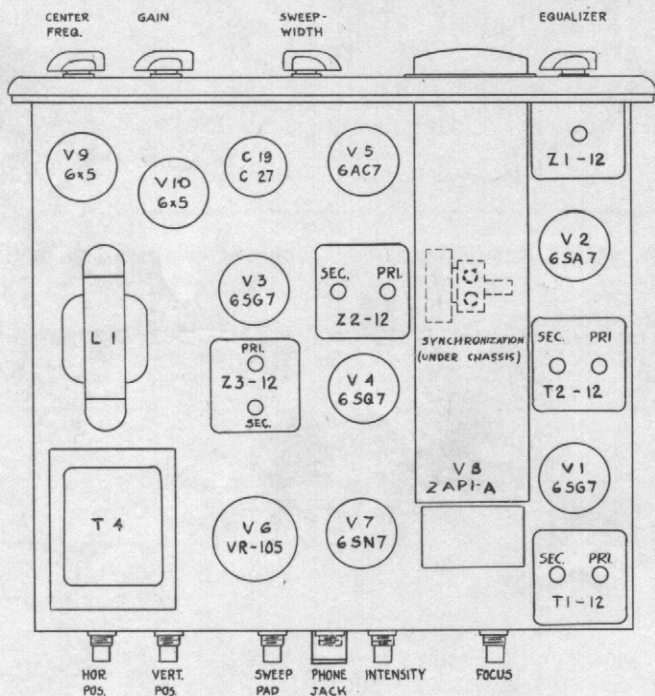
Figure 34. Top View of Chassis
