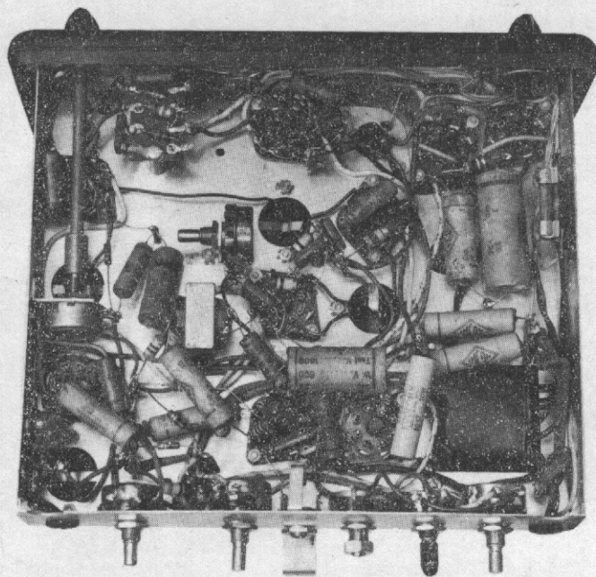
Figure 35. Bottom View of Chassis
